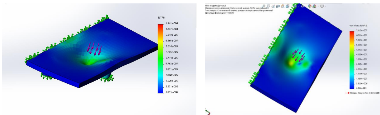
Fig. 2. Component part relocation under the effect of 1000 N cutting force Fig. 3. Stresses in component part under 1000 N cutting force
